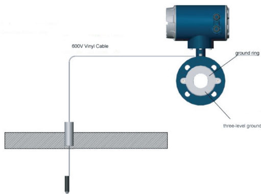
Figure 13 Instrument grounding
