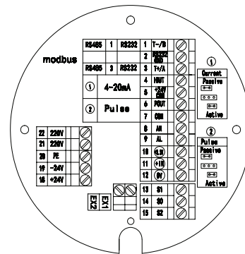
Figure 3 Integrated wiring diagram
