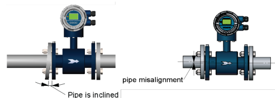
Figure 12 Flowmeter installation symmetrically with the pipe axis
